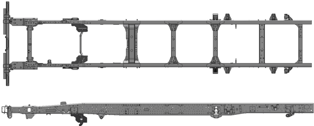
Figure 12: NQR & NRR Gas Frame
