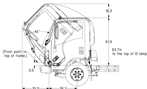
Figure 15: N-Series Gas Cab Tilt Dimensions
