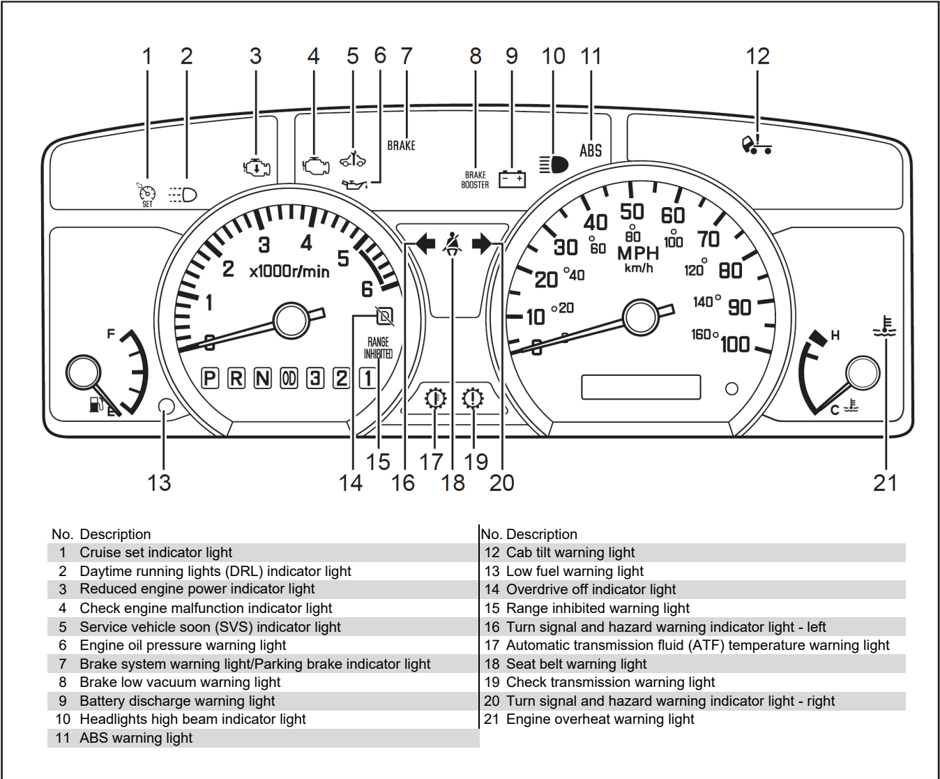
Figure 24: N-Series Gas Instrument Panel, Warning lights and indicators
