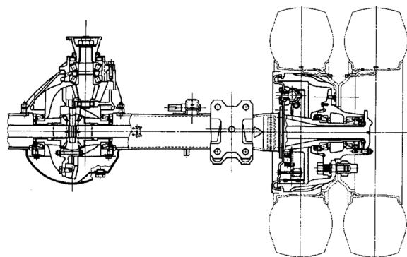
Figure 9: NQR &amp; NRR Gas Rear Axle
