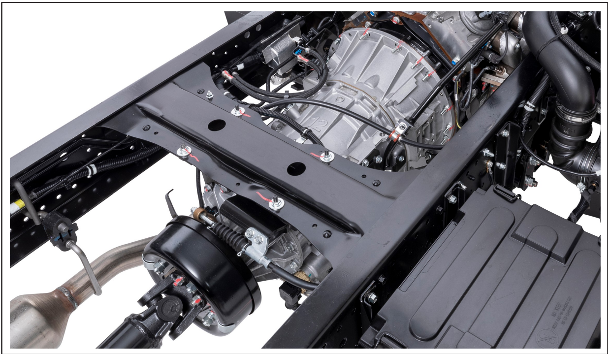
Figure 4: NQR & NRR Gas Allison RDS 1000 Transmission
