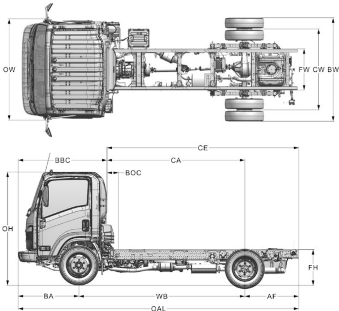
Figure 1: NQR and NRR Gas Standard Cab Chassis Dimensions
