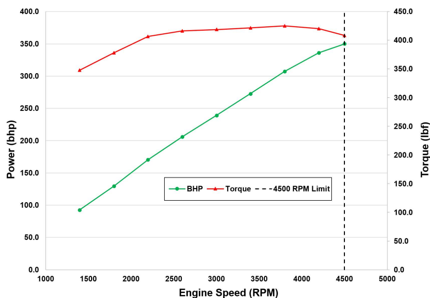
Figure 3: N-Series Gas Engine Performance Curve
