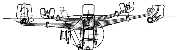
Figure 10: NQR &amp; NRR Gas Rear Suspension
