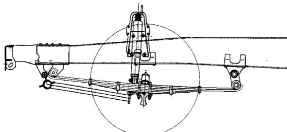
Figure 6: NQR & NRR Gas Front Suspension
