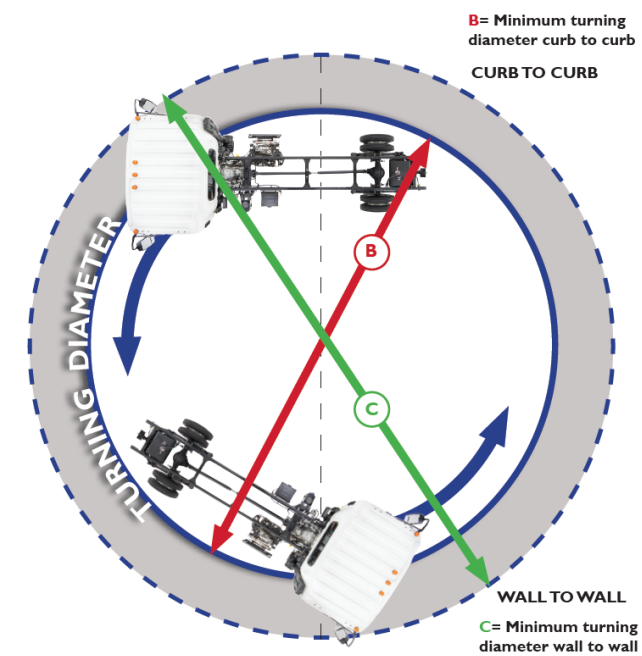
Figure 8: NQR & NRR Gas Turning Circle
