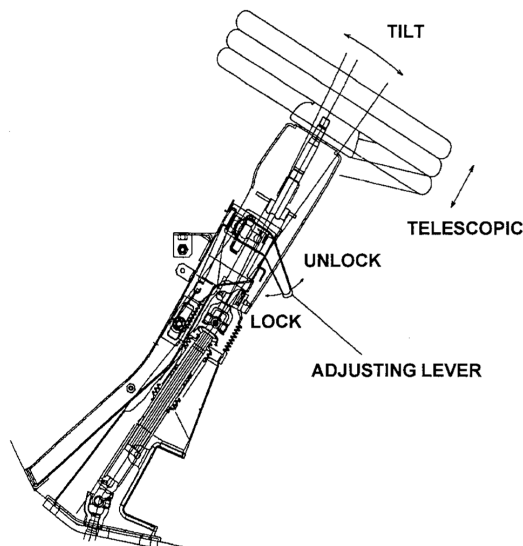
Figure 21: N-Series Steering Column
